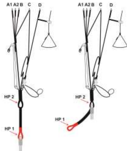
Fig. 6: Hangpoint
