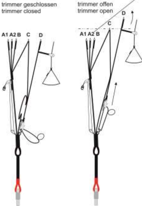
Fig. 9: how the trimmers work
