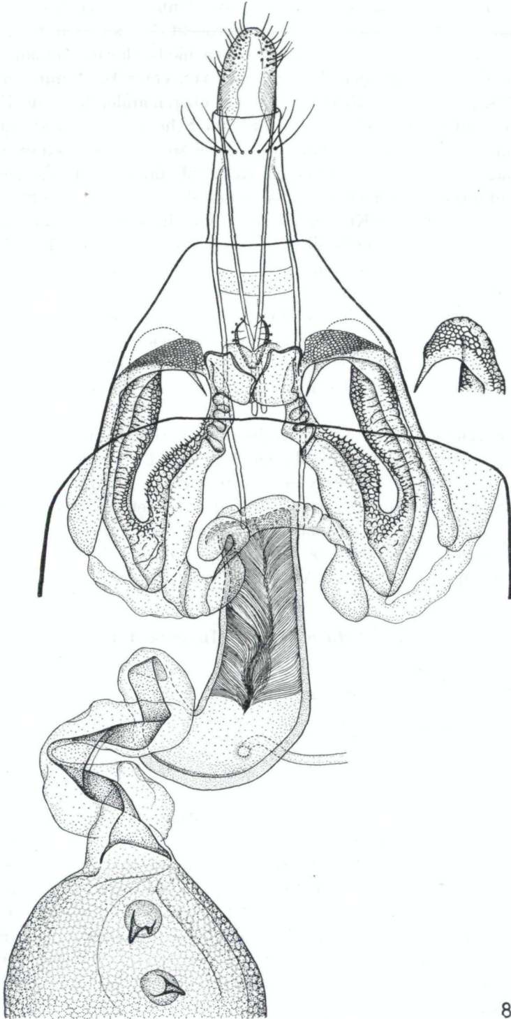
Abb. 8. Calycobathra striatella n. sp., ♀-Genital; GU-4183-Amsel.
